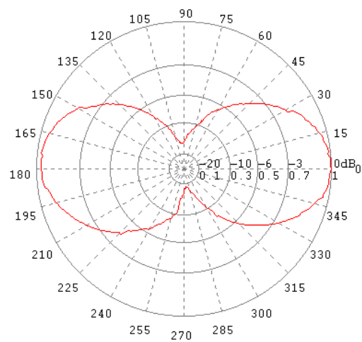
E-Ebene / E-Plane 90 MHz
