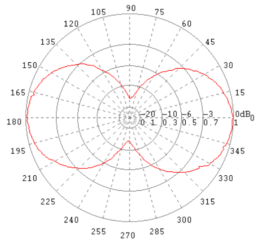
E-Ebene / E-Plane 30 MHz
