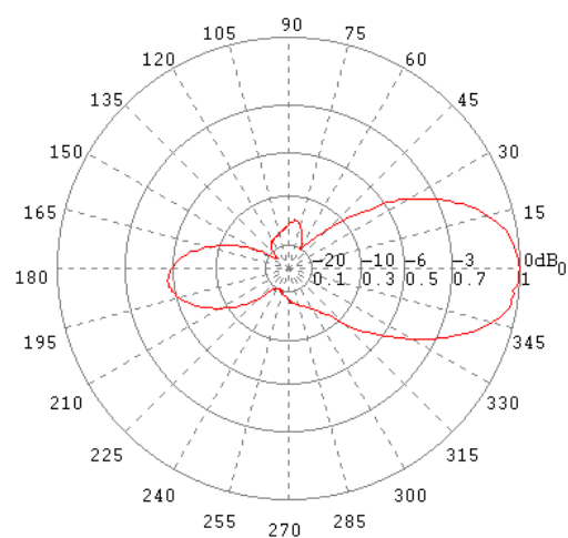
E-Ebene / E-Plane 150 MHz
