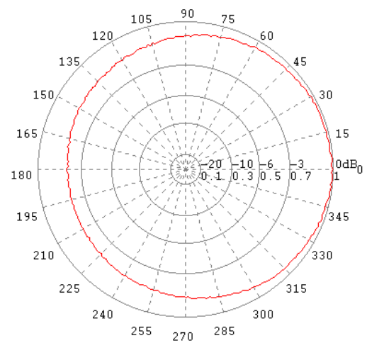
H-Ebene / H-Plane 90 MHz
