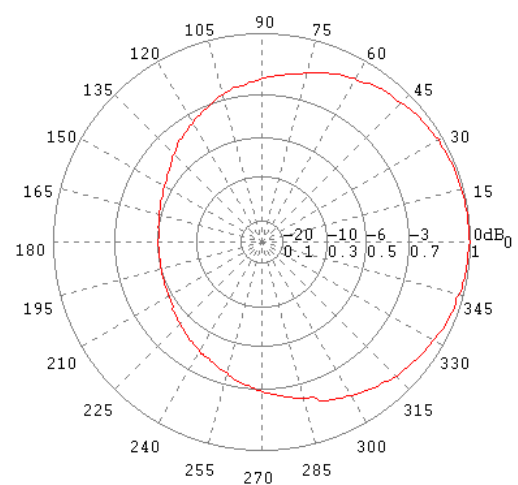
H-Ebene / H-Plane 150 MHz
