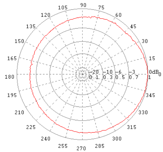
H-Ebene / H-Plane 30 MHz
