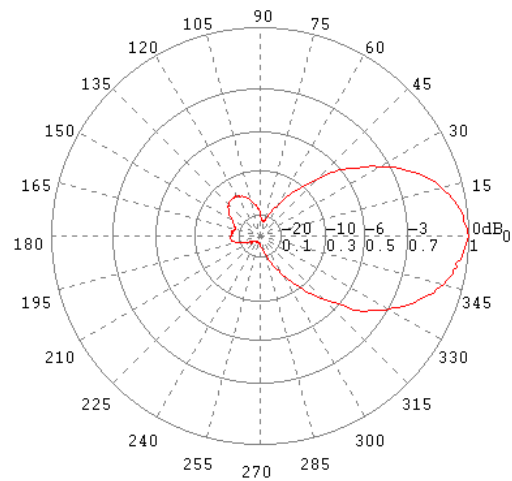
E-Ebene / E-Plane 200 MHz
