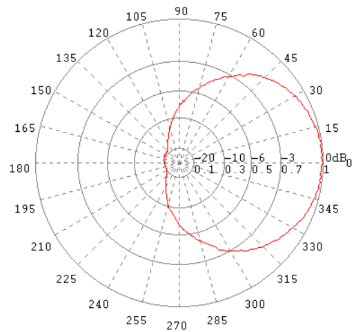
H-Ebene / H-Plane 200 MHz
