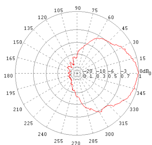
H-Ebene / H-Plane 1000 MHz
