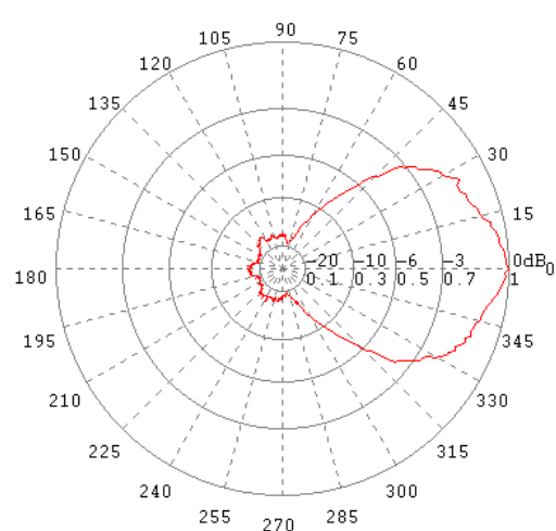
E-Ebene / E-Plane 1000 MHz
